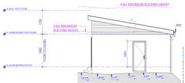
SOUTH ELEVATION
