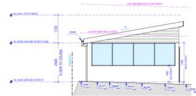
NORTH ELEVATION
