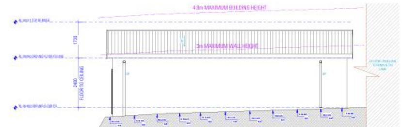
EAST ELEVATION
