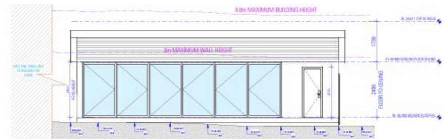
WEST ELEVATION
